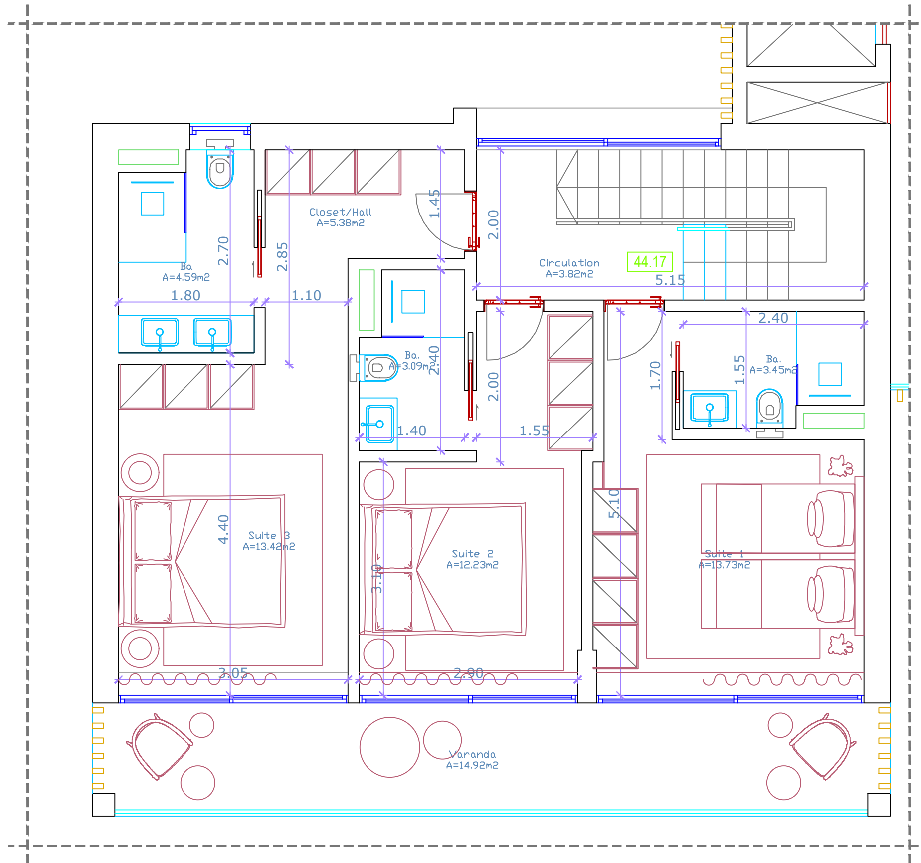
APARTMENT PLAN (LOWER FLOOR)
