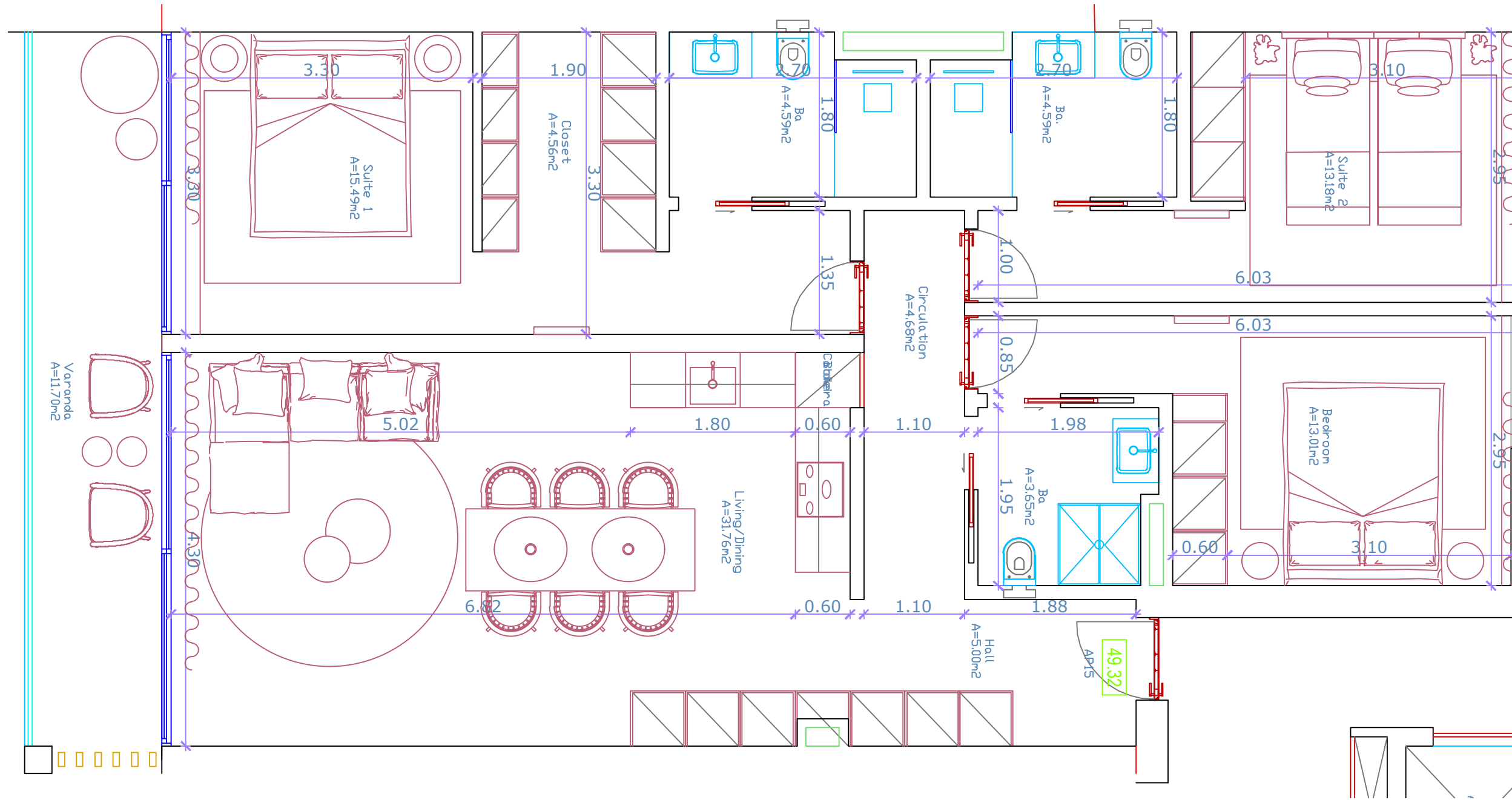
APARTMENT PLAN
